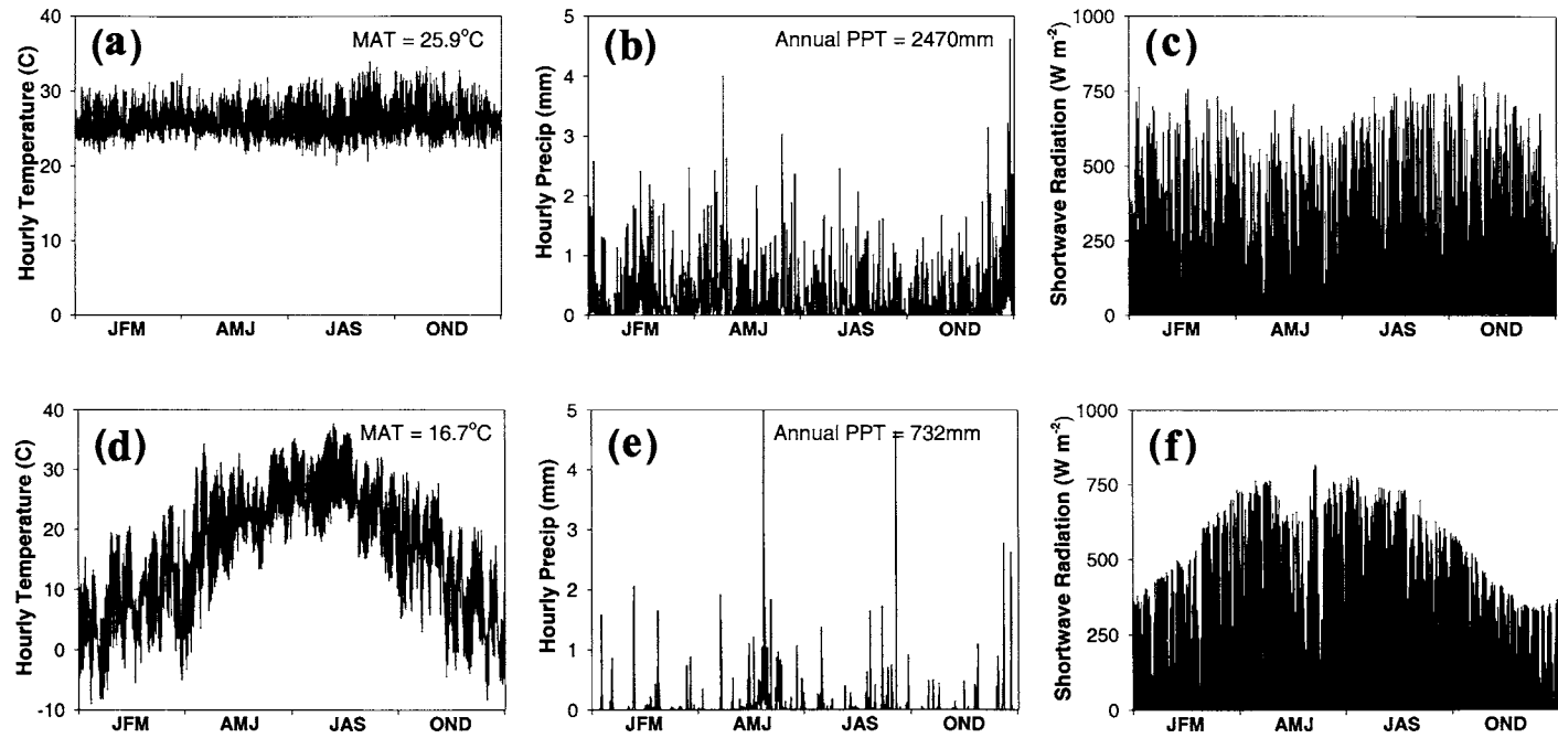
Figure 1. Hourly input climate data for TerraFlux simulations of a lowland humid tropical forest and a semi-arid savanna/grassland. These datasets are taken from the ECMWF Climate Reanalysis (ECMWF 1998). (a)–(c) Temperature, rainfall, and downwelling solar radiation from 1990 at 3°S, 60°W (West-Central Amazon Basin). (d)–(f) Temperature, rainfall, and downwelling solar radiation from 1990 at 34°N, 99°W (North Texas mesquite savanna). MAT = mean annual temperature.
