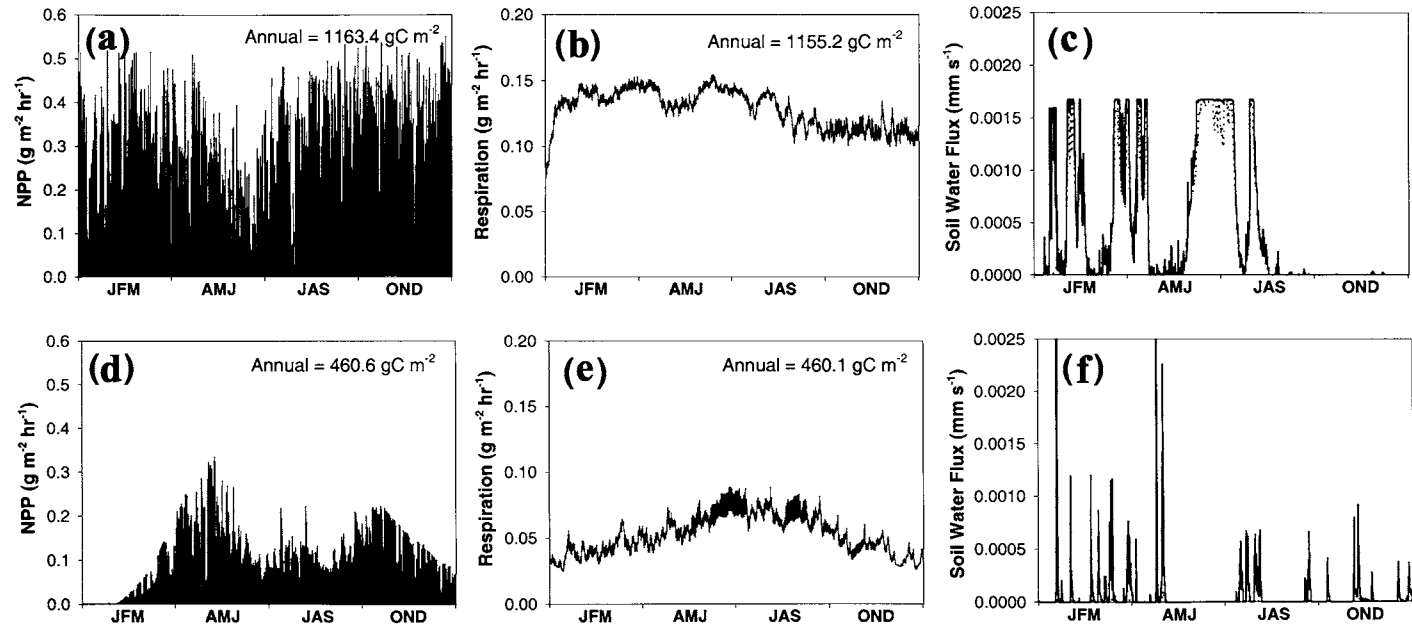
Figure 2. Hourly NPP, heterotrophic respiration, and soil water flux at 0–10/10–30cm depths at the end of the model spin up, prior to the onset of 50 years of \text{NO}_3^- deposition. (a)–(c) Lowland humid tropical forest. (d)–(f) Semi-arid savanna/grassland.
